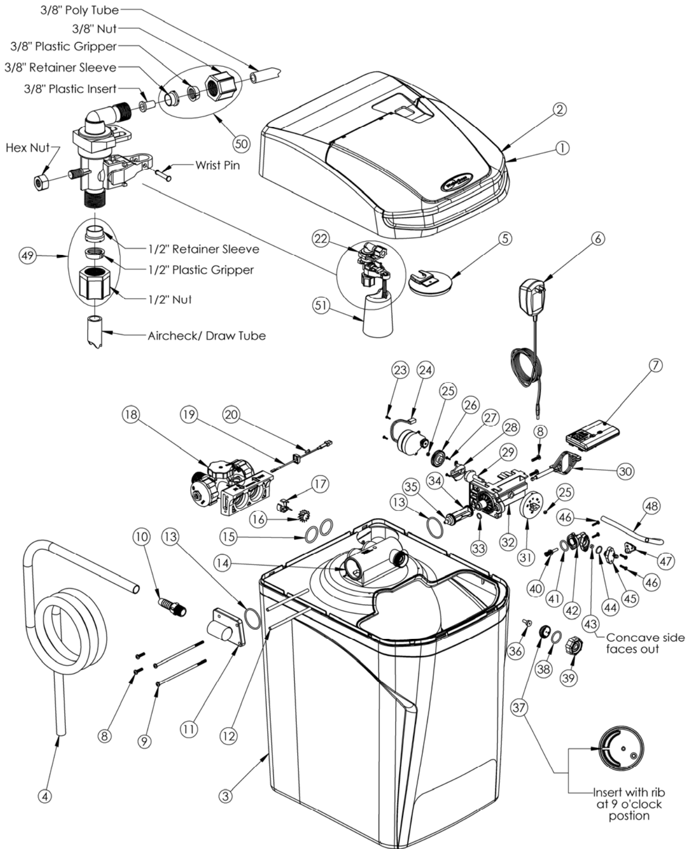
Figure 10: Cabinet and Assemblies
