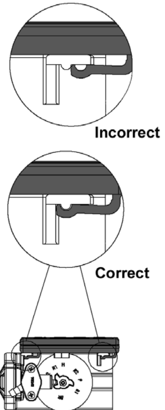
Figure 8: Controller Tab Lock Detail
