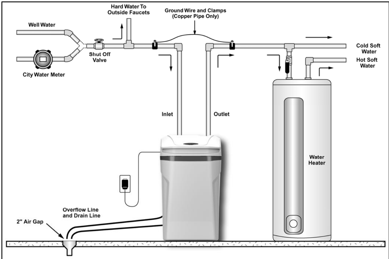
Figure 1: Appliance Placement
