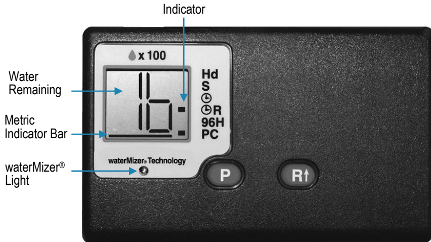
Figure 7: Two-Button Controller
