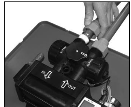
Figure 3: Connect Water Lines
