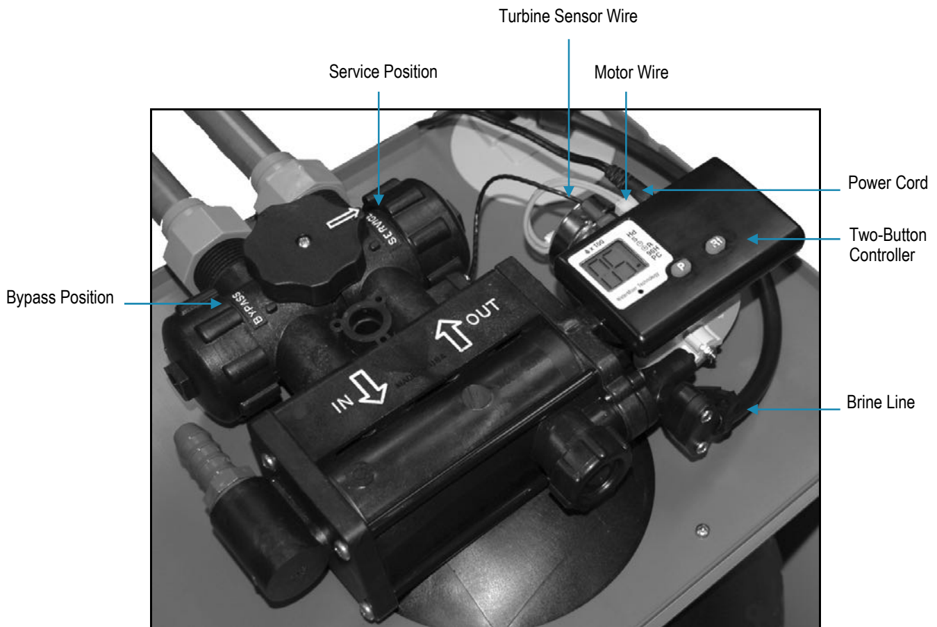
Figure 6: Valve View of Softener
